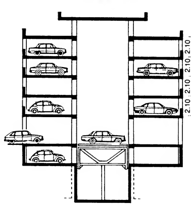
⑬ Cross-section → ⑪
